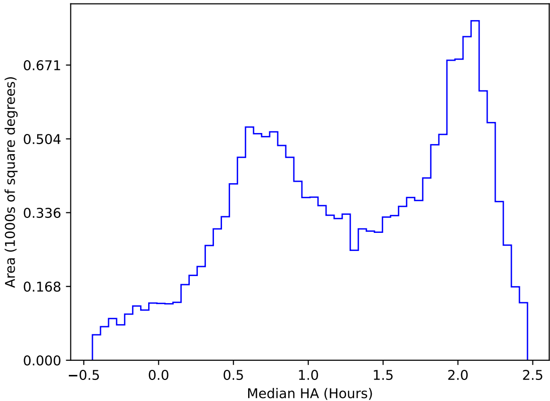
too_elab_r64_d2_ugrizy_v3.4_10yrs WFD y band: Median HA
