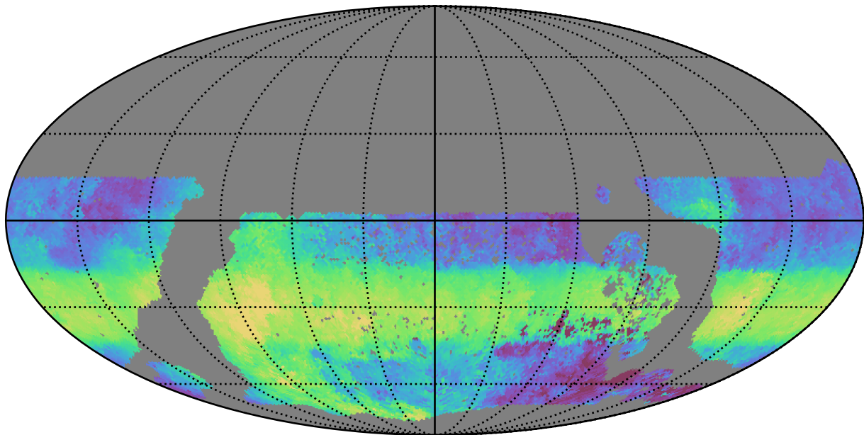
too_elab_r64_d2_ugrizy_v3.4_10yrs WFD u band: Median HA
