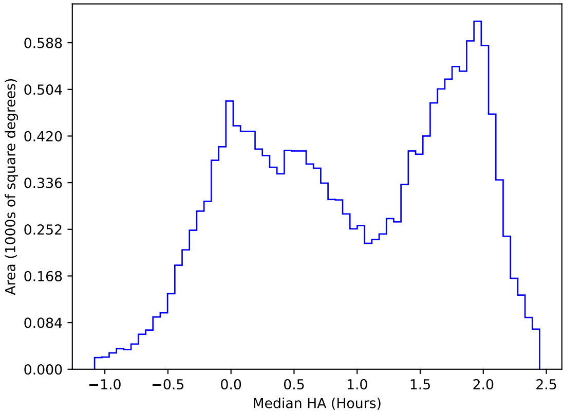
too_elab_r64_d2_ugrizy_v3.4_10yrs WFD u band: Median HA
