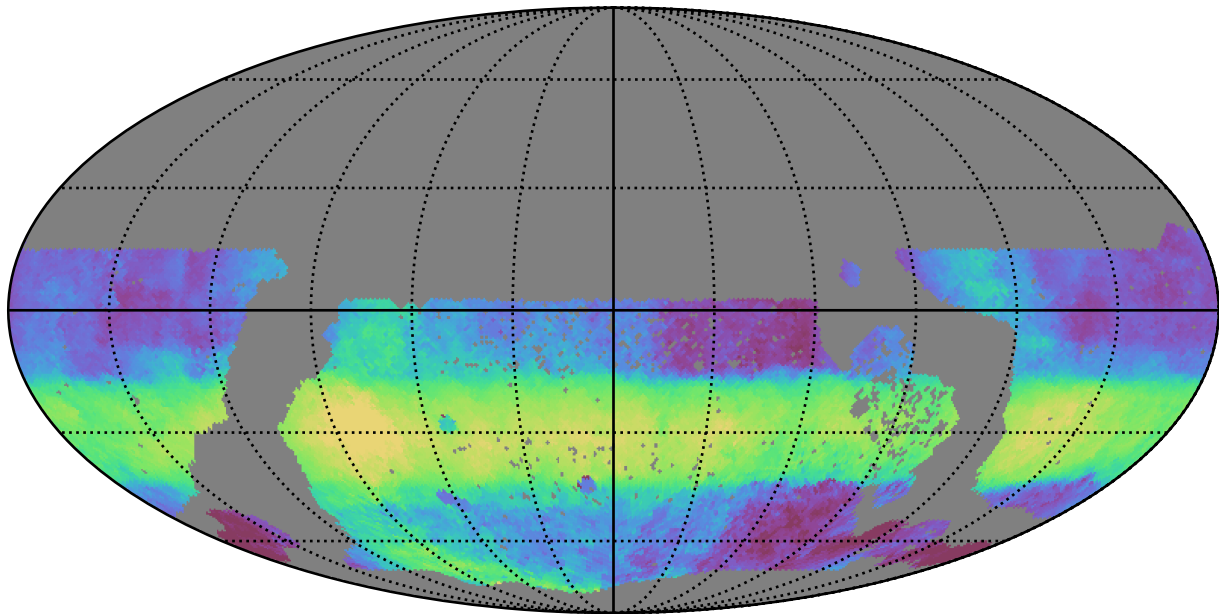
too_elab_r64_d2_ugrizy_v3.4_10yrs WFD r band: Median HA
