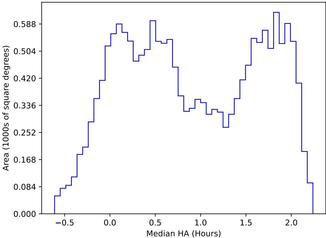
too_elab_r64_d2_ugrizy_v3.4_10yrs WFD r band: Median HA
