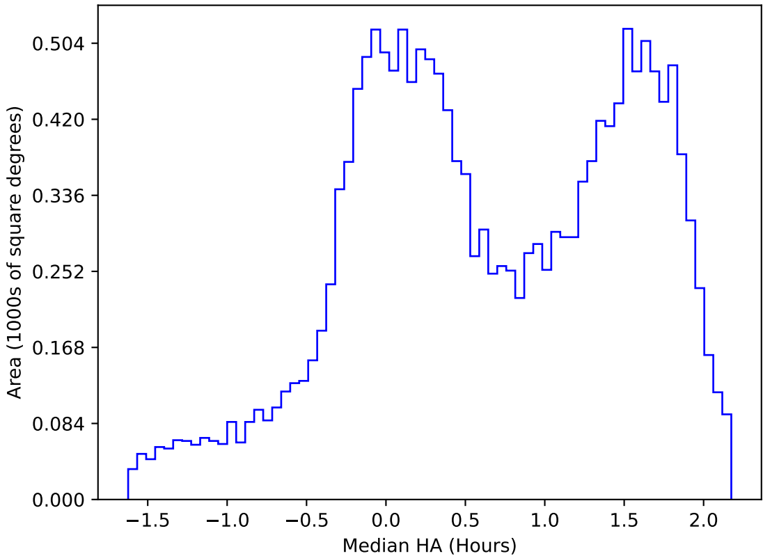
too_elab_r64_d2_ugrizy_v3.4_10yrs WFD g band: Median HA
