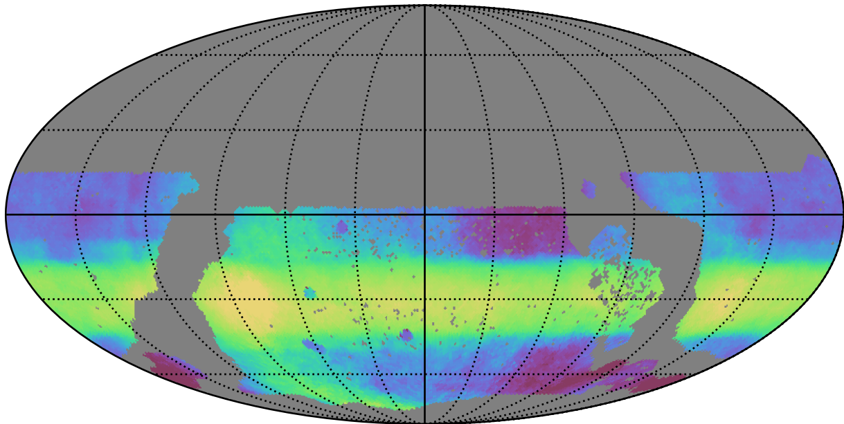
too_elab_r64_d2_ugrizy_v3.4_10yrs WFD all bands: Median HA
