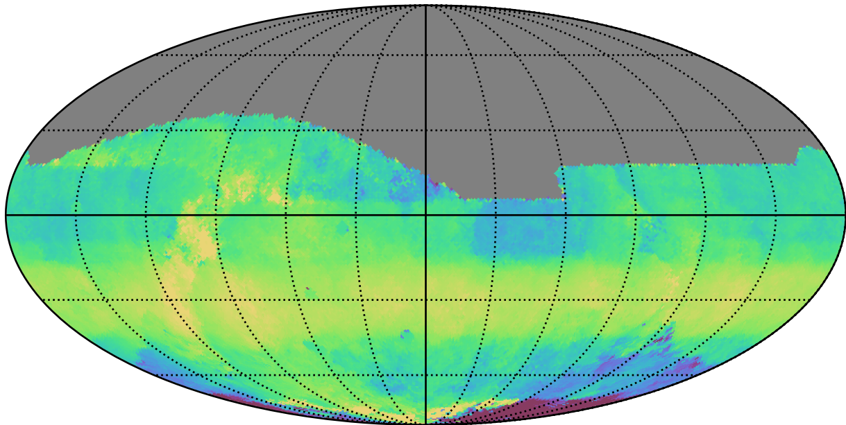
too_elab_r64_d2_ugrizy_v3.4_10yrs All sky z band: Median HA
