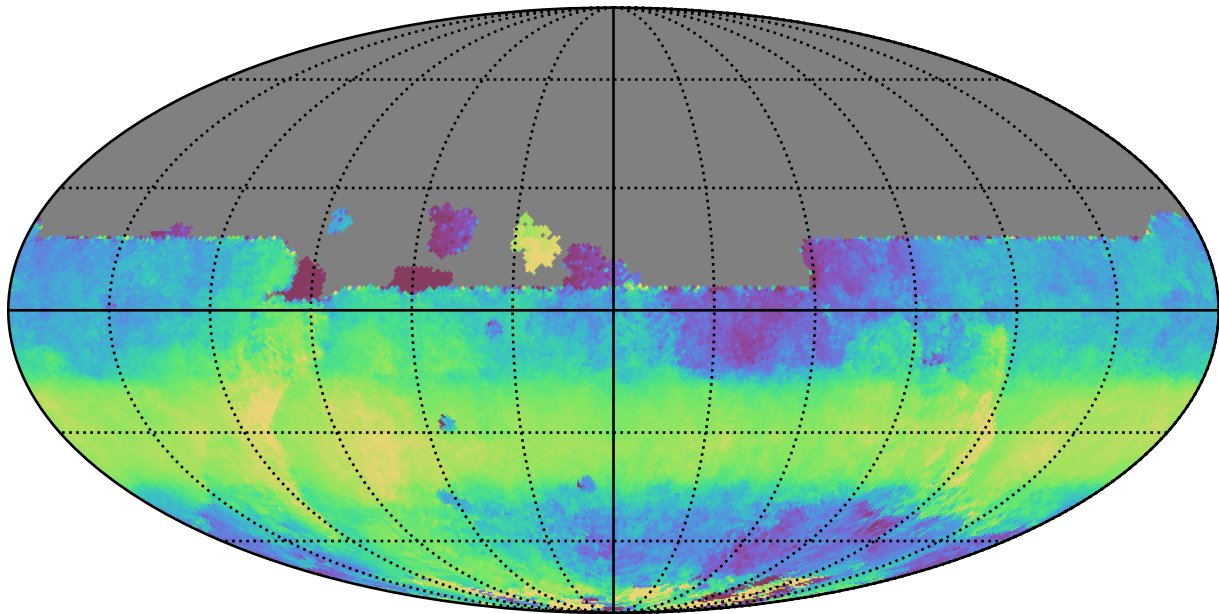
too_elab_r64_d2_ugrizy_v3.4_10yrs All sky y band: Median HA
