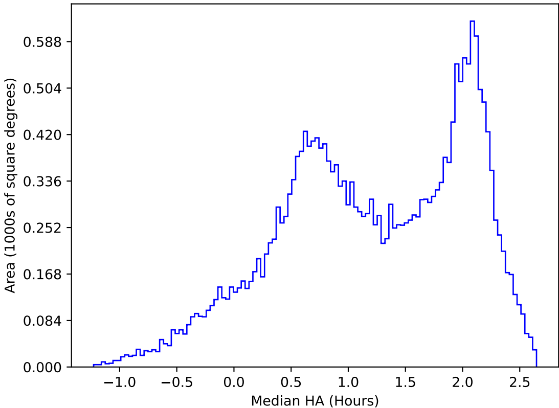
too_elab_r64_d2_ugrizy_v3.4_10yrs All sky y band: Median HA
