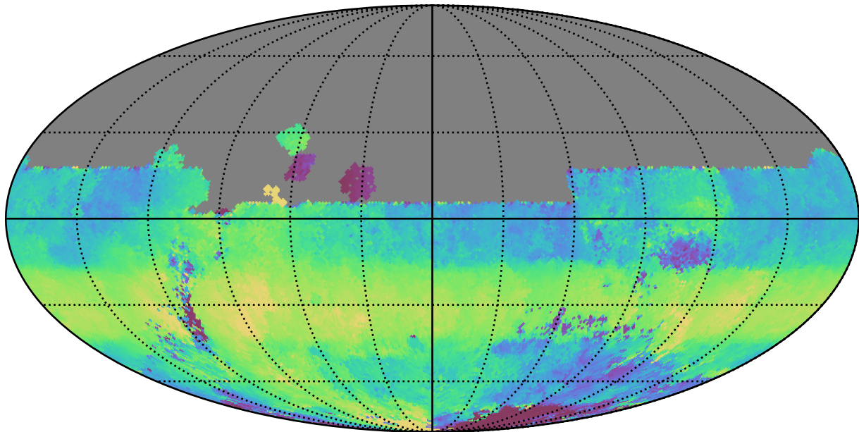
too_elab_r64_d2_ugrizy_v3.4_10yrs All sky u band: Median HA
