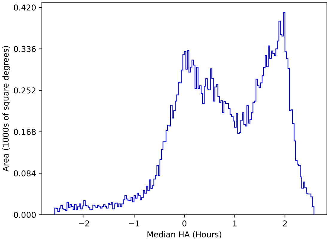
too_elab_r64_d2_ugrizy_v3.4_10yrs All sky u band: Median HA
