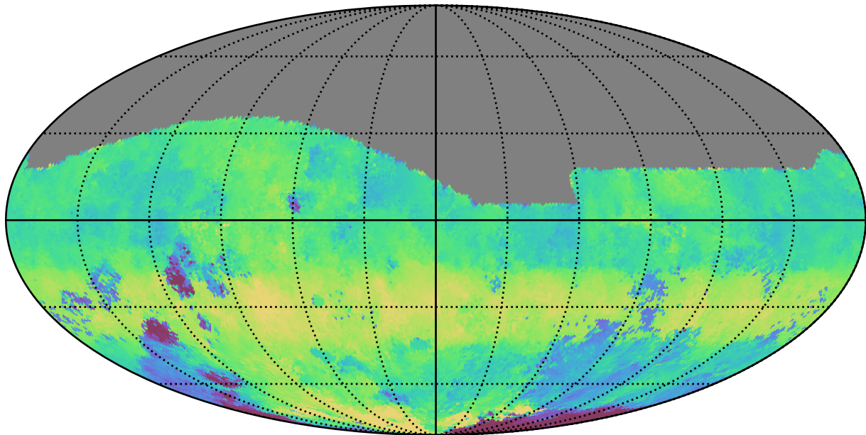
too_elab_r64_d2_ugrizy_v3.4_10yrs All sky g band: Median HA
