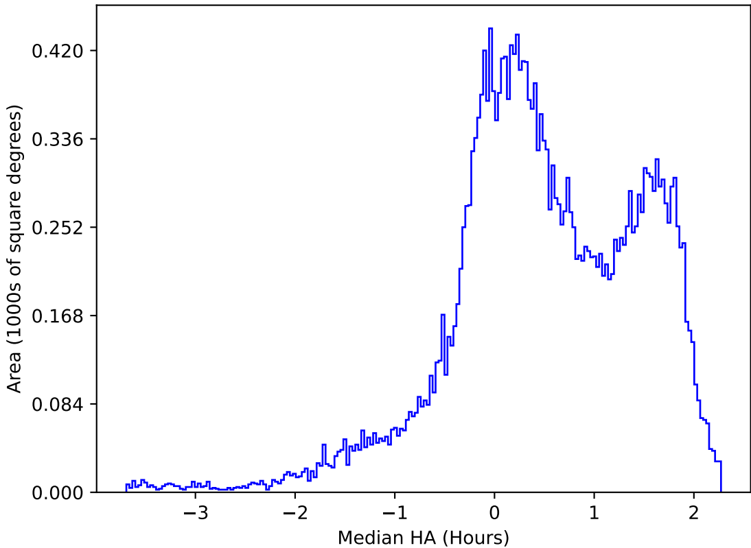
too_elab_r64_d2_ugrizy_v3.4_10yrs All sky g band: Median HA
