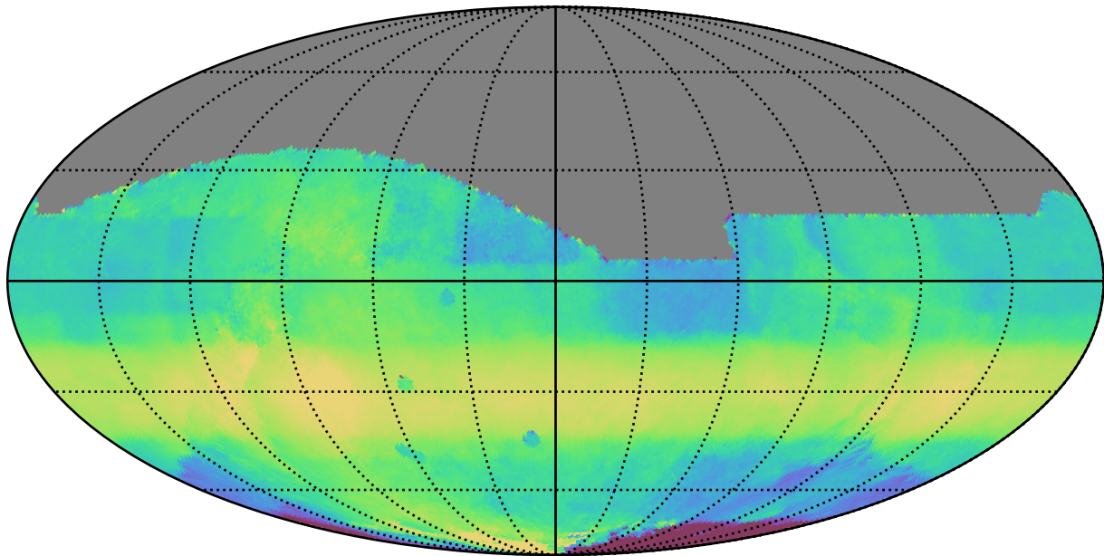
too_elab_r64_d2_ugrizy_v3.4_10yrs All sky all bands: Median HA
