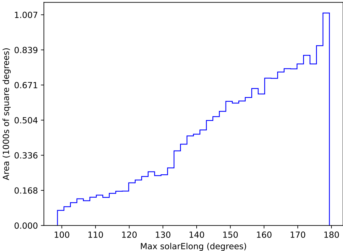
too_elab_r64_d2_ugrizy_v3.4_10yrs WFD z band: Max solarElong
