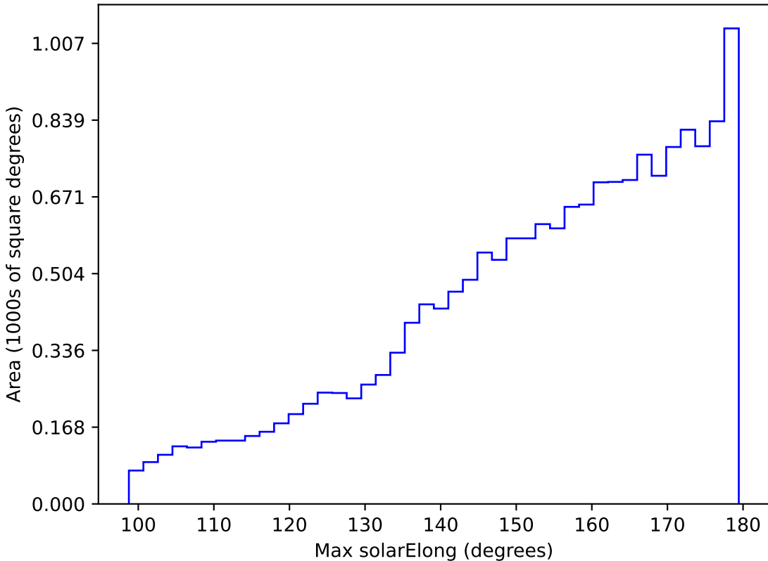
too_elab_r64_d2_ugrizy_v3.4_10yrs WFD r band: Max solarElong
