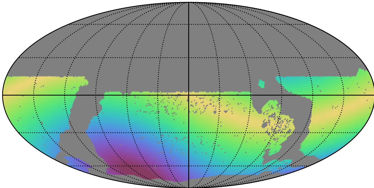
too_elab_r64_d2_ugrizy_v3.4_10yrs WFD i band: Max solarElong
