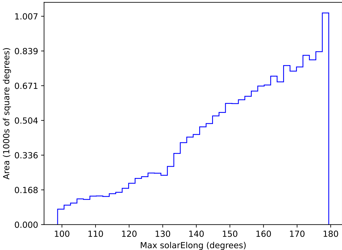
too_elab_r64_d2_ugrizy_v3.4_10yrs WFD i band: Max solarElong
