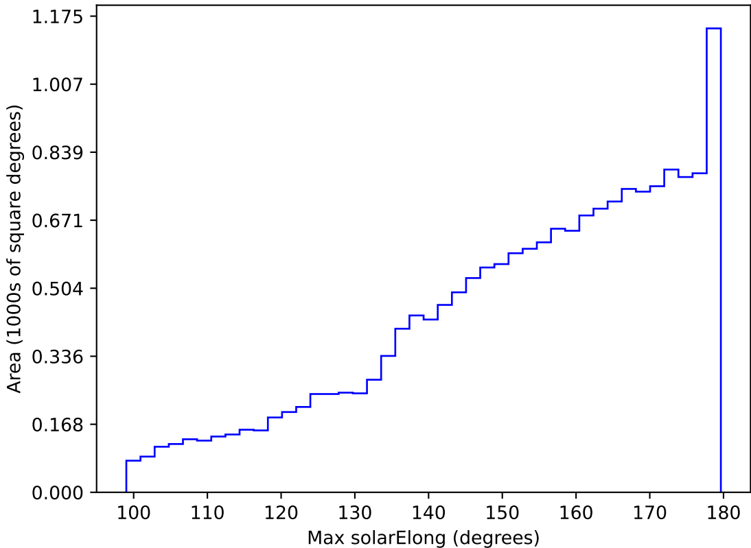
too_elab_r64_d2_ugrizy_v3.4_10yrs WFD all bands: Max solarElong
