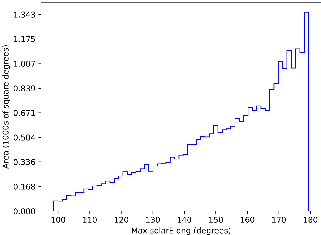
too_elab_r64_d2_ugrizy_v3.4_10yrs All sky r band: Max solarElong
