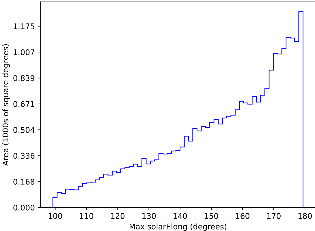
too_elab_r64_d2_ugrizy_v3.4_10yrs All sky i band: Max solarElong
