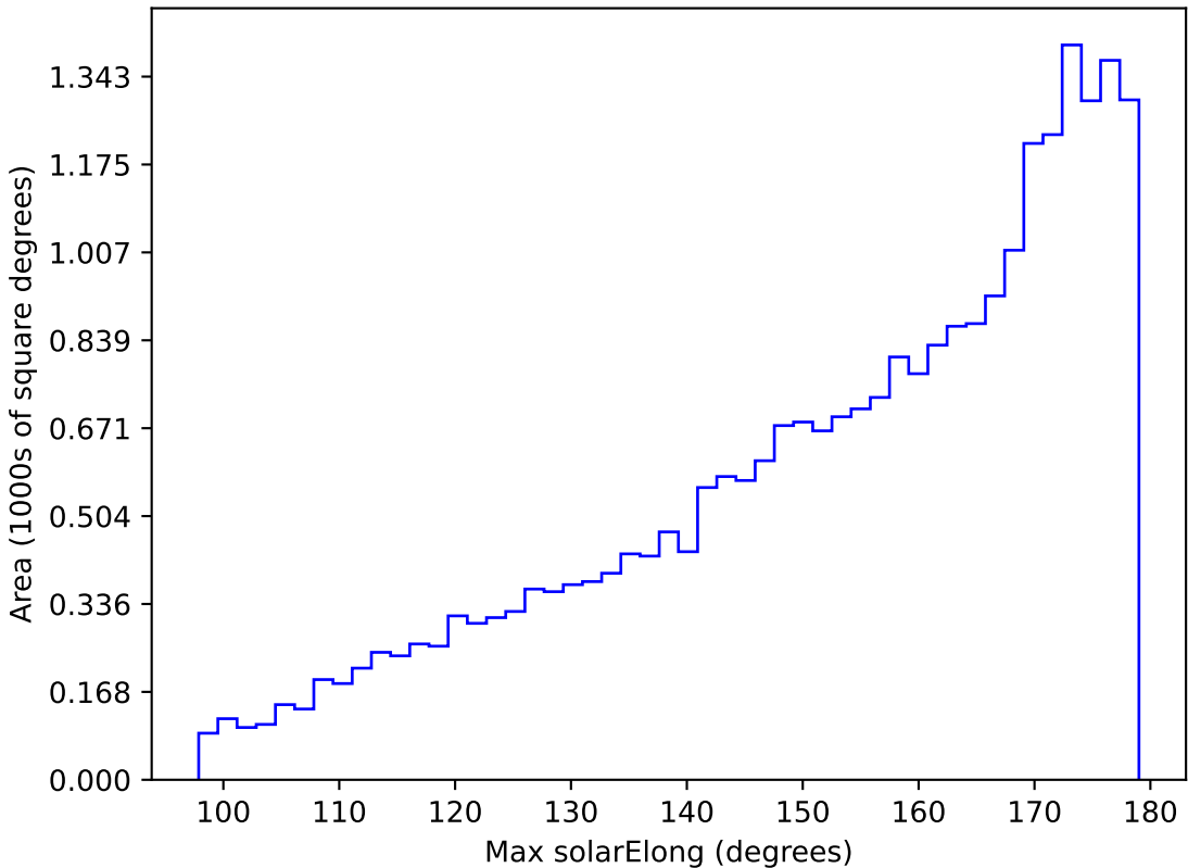
too_elab_r64_d2_ugrizy_v3.4_10yrs All sky g band: Max solarElong
