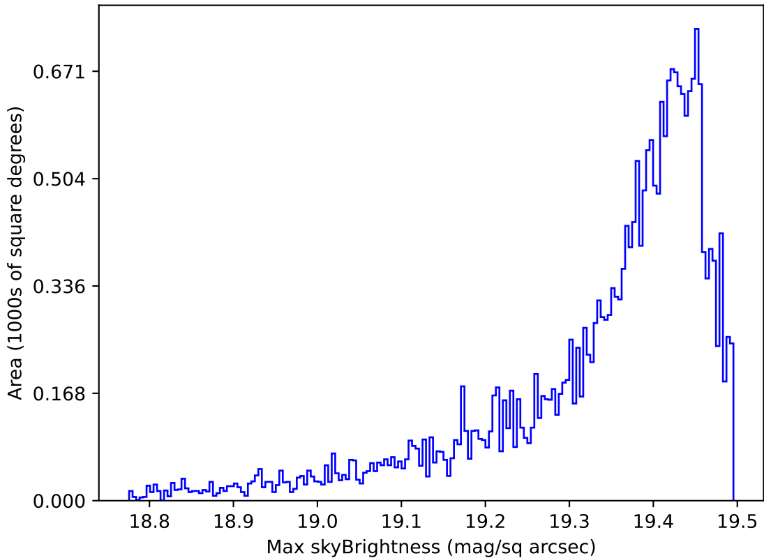
too_elab_r64_d2_ugrizy_v3.4_10yrs Yr 1 z band: Max skyBrightness
