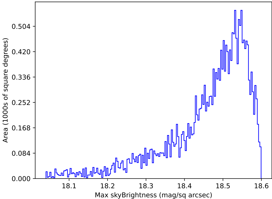
too_elab_r64_d2_ugrizy_v3.4_10yrs Yr 1 y band: Max skyBrightness
