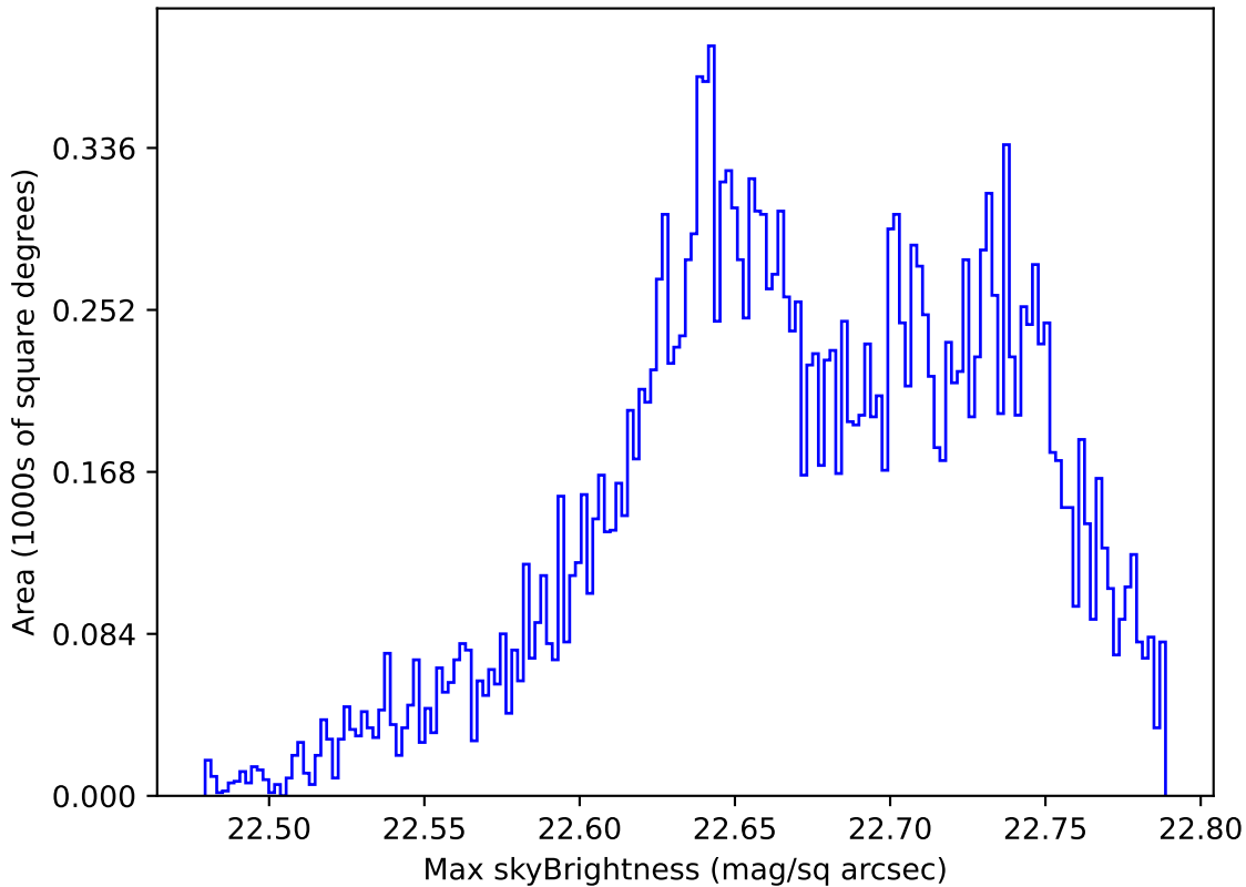
too_elab_r64_d2_ugrizy_v3.4_10yrs Yr 1 u band: Max skyBrightness
