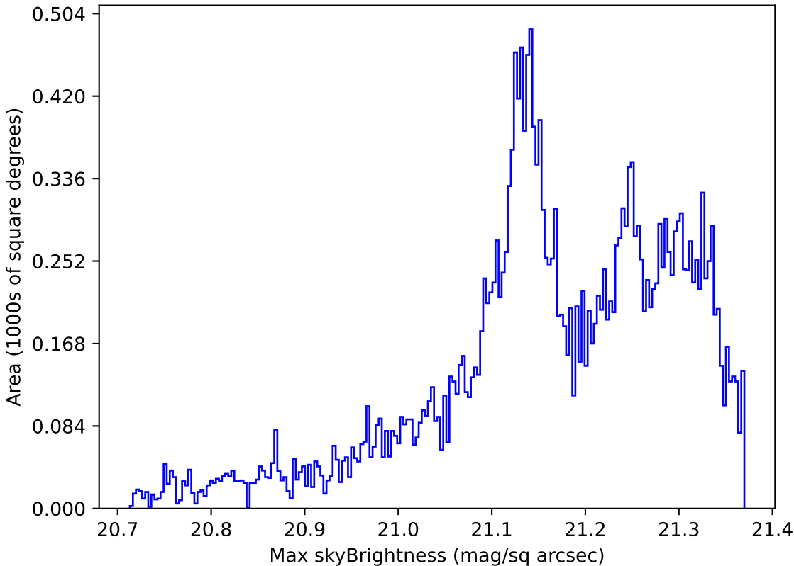
too_elab_r64_d2_ugrizy_v3.4_10yrs Yr 1 r band: Max skyBrightness
