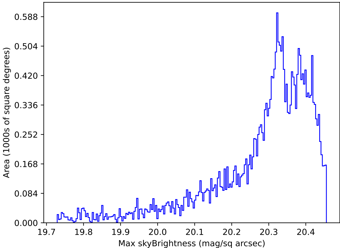
too_elab_r64_d2_ugrizy_v3.4_10yrs Yr 1 i band: Max skyBrightness
