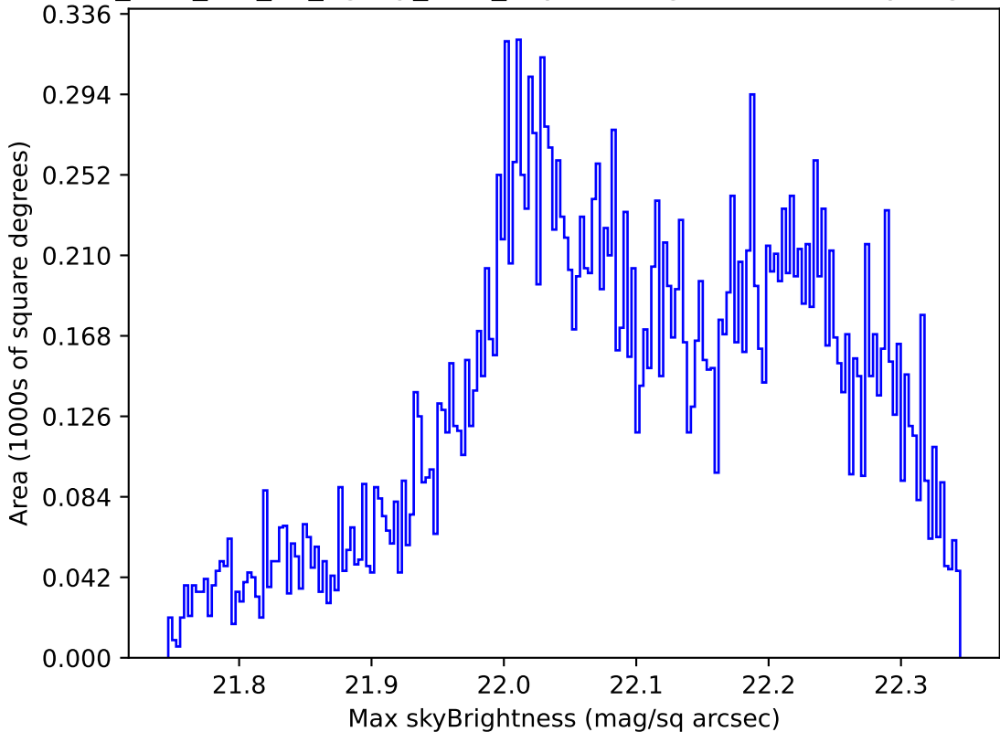
too_elab_r64_d2_ugrizy_v3.4_10yrs Yr 1 g band: Max skyBrightness
