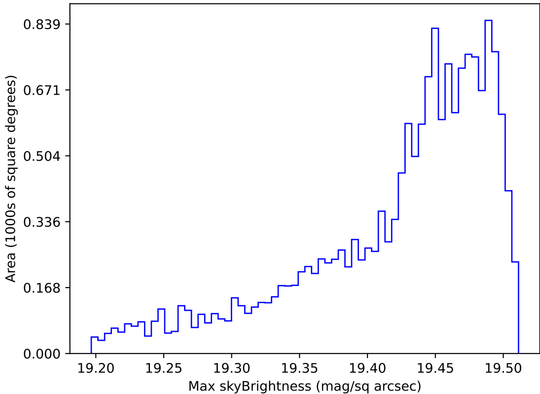
too_elab_r64_d2_ugrizy_v3.4_10yrs WFD z band: Max skyBrightness
