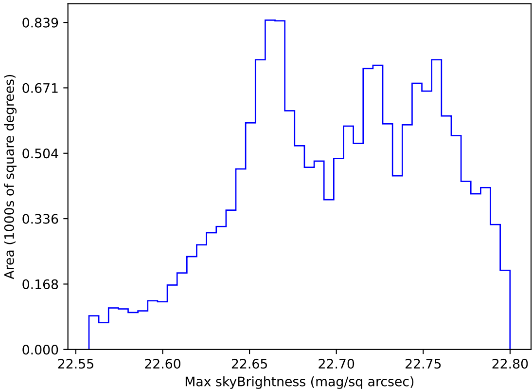
too_elab_r64_d2_ugrizy_v3.4_10yrs WFD u band: Max skyBrightness
