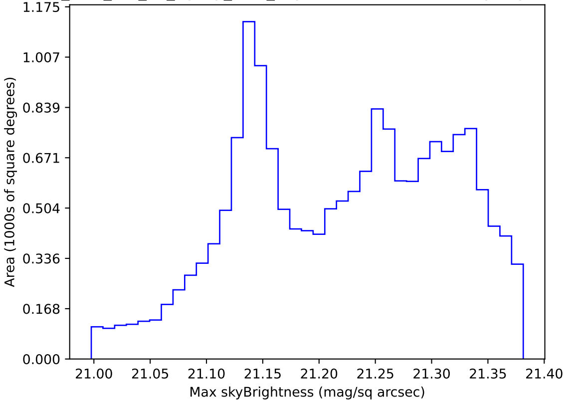
too_elab_r64_d2_ugrizy_v3.4_10yrs WFD r band: Max skyBrightness
