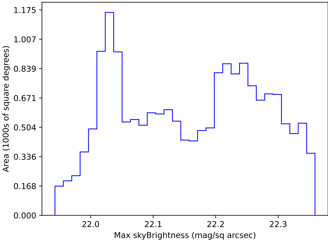
too_elab_r64_d2_ugrizy_v3.4_10yrs WFD g band: Max skyBrightness
