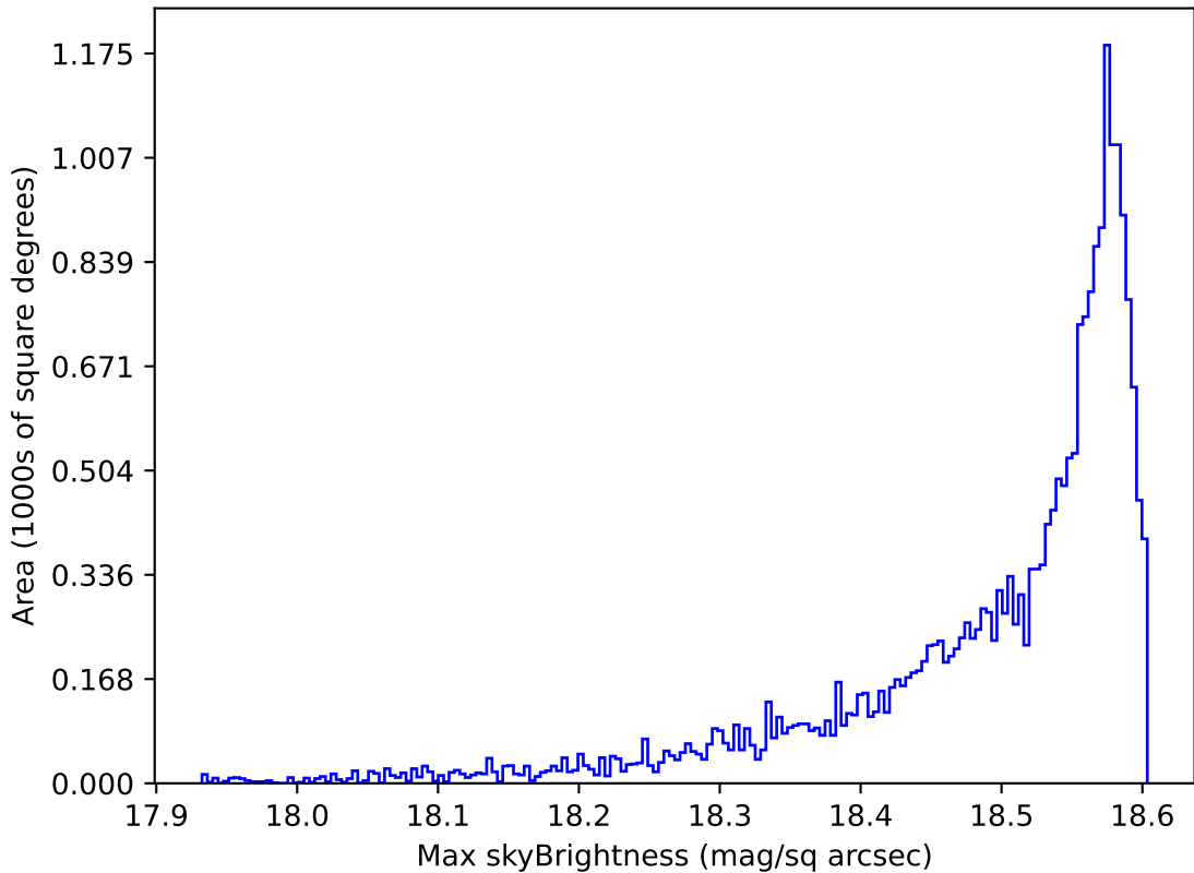
too_elab_r64_d2_ugrizy_v3.4_10yrs All sky y band: Max skyBrightness
