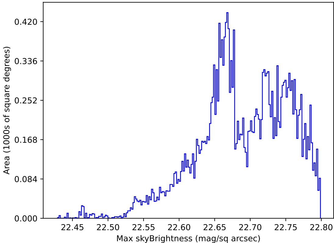
too_elab_r64_d2_ugrizy_v3.4_10yrs All sky u band: Max skyBrightness
