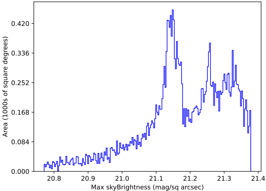
too_elab_r64_d2_ugrizy_v3.4_10yrs All sky r band: Max skyBrightness
