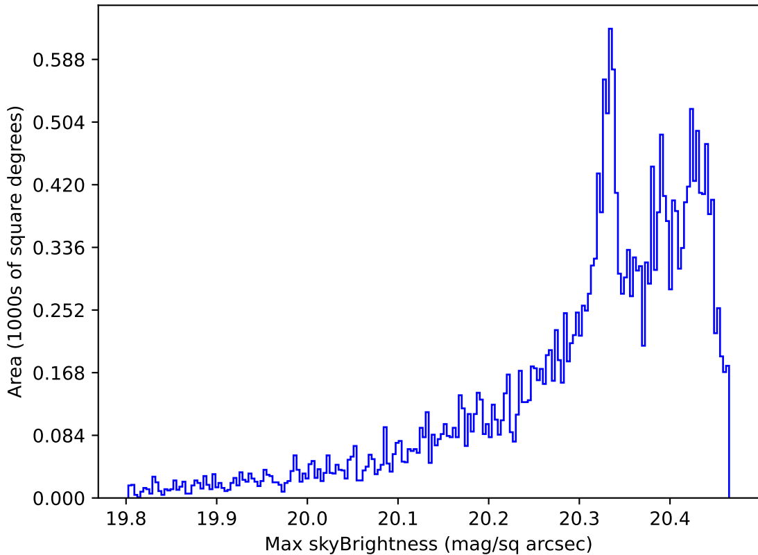
too_elab_r64_d2_ugrizy_v3.4_10yrs All sky i band: Max skyBrightness
