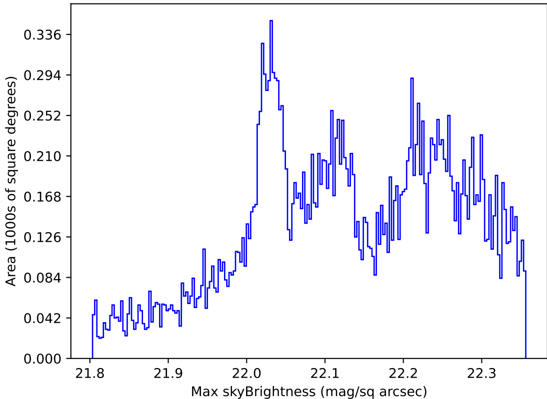
too_elab_r64_d2_ugrizy_v3.4_10yrs All sky g band: Max skyBrightness
