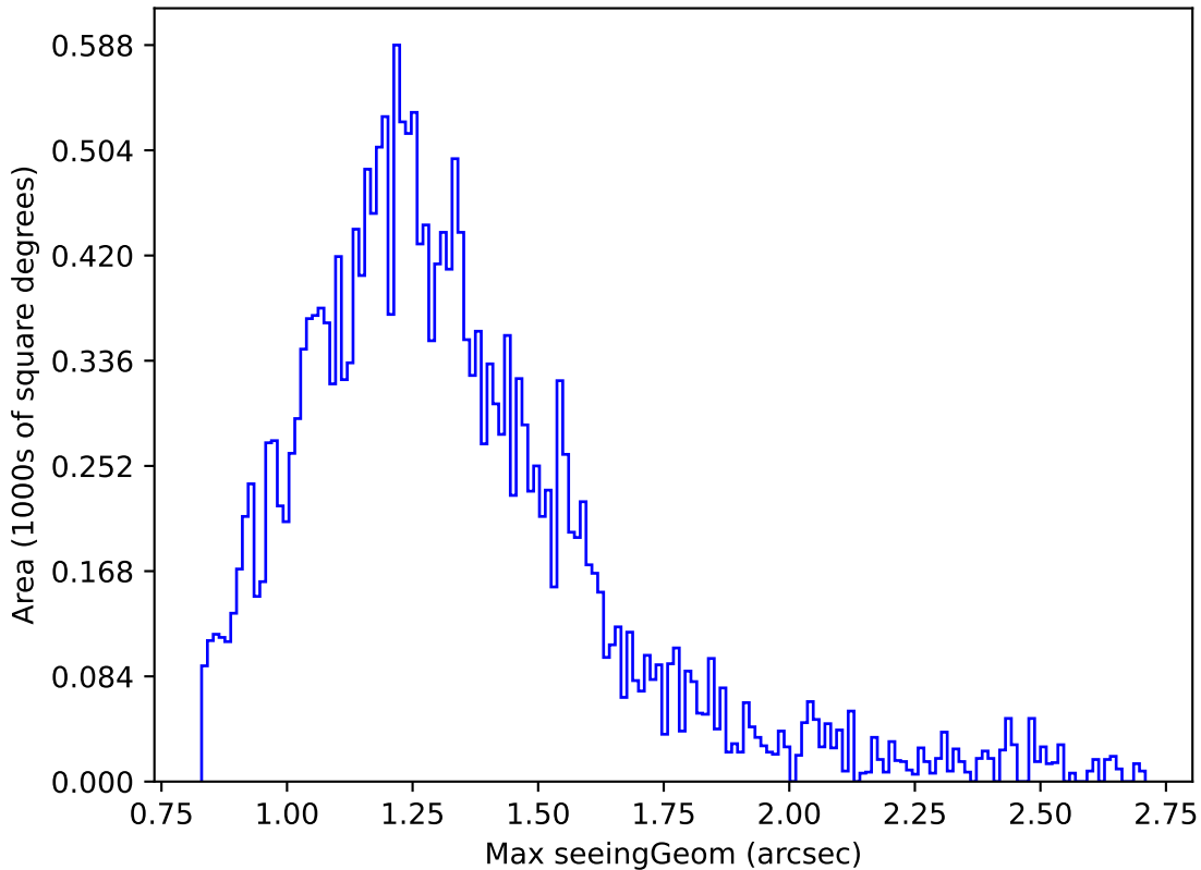
too_elab_r64_d2_ugrizy_v3.4_10yrs Yr 1 u band: Max seeingGeom
