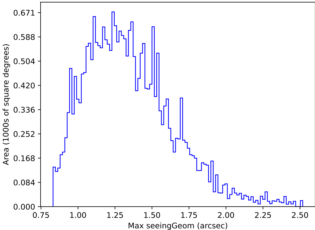
too_elab_r64_d2_ugrizy_v3.4_10yrs Yr 1 r band: Max seeingGeom
