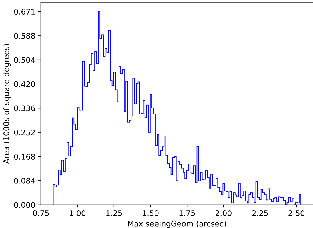
too_elab_r64_d2_ugrizy_v3.4_10yrs Yr 1 i band: Max seeingGeom
