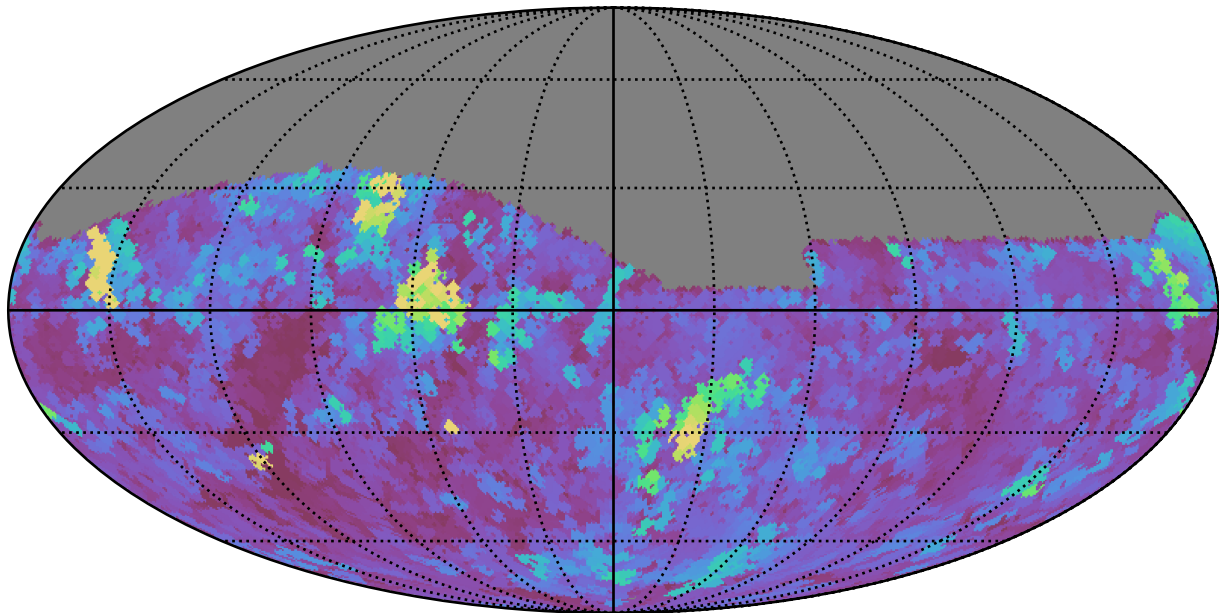
too_elab_r64_d2_ugrizy_v3.4_10yrs Yr 1 z band: Max seeingEff
