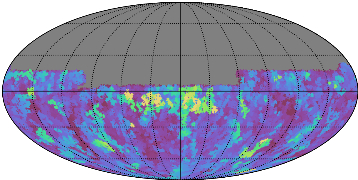
too_elab_r64_d2_ugrizy_v3.4_10yrs Yr 1 y band: Max seeingEff
