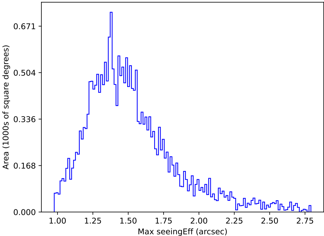
too_elab_r64_d2_ugrizy_v3.4_10yrs Yr 1 y band: Max seeingEff
