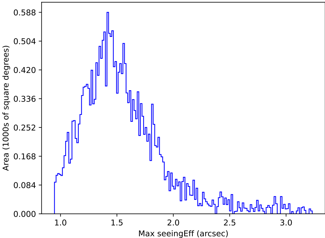
too_elab_r64_d2_ugrizy_v3.4_10yrs Yr 1 u band: Max seeingEff
