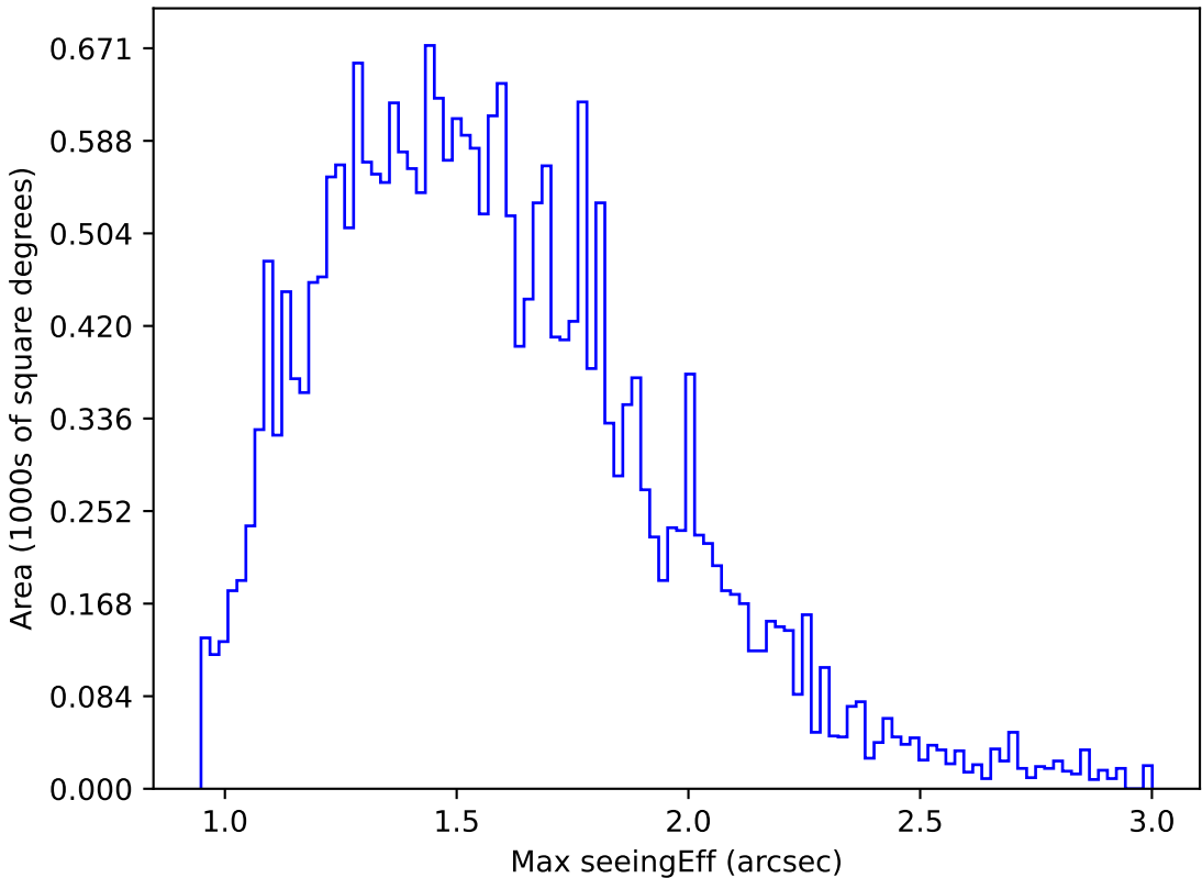
too_elab_r64_d2_ugrizy_v3.4_10yrs Yr 1 r band: Max seeingEff
