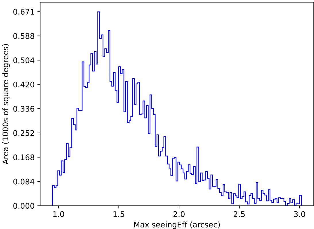
too_elab_r64_d2_ugrizy_v3.4_10yrs Yr 1 i band: Max seeingEff
