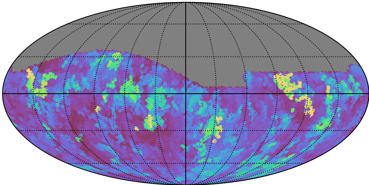
too_elab_r64_d2_ugrizy_v3.4_10yrs Yr 1 all bands: Max seeingEff
