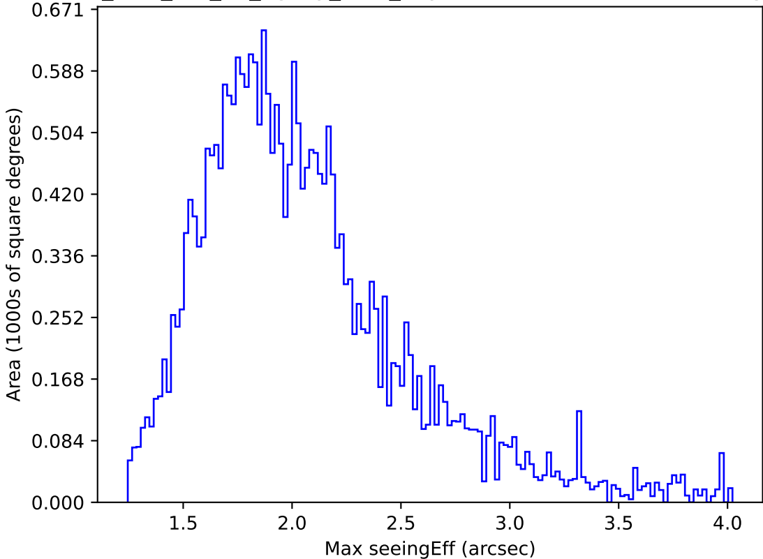
too_elab_r64_d2_ugrizy_v3.4_10yrs Yr 1 all bands: Max seeingEff
