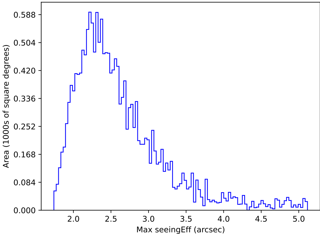
too_elab_r64_d2_ugrizy_v3.4_10yrs WFD z band: Max seeingEff
